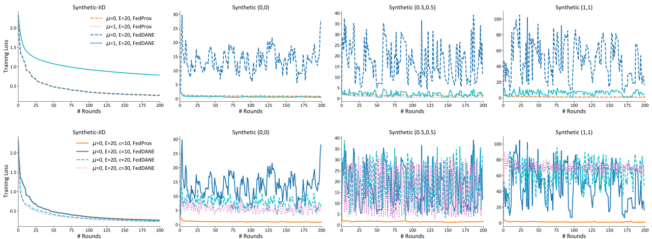
Figure 4. DANE and AIDE (Shamir et al., 2014; Reddi et al., 2016) are methods proposed in the data center setting that use a similar proximal term as \text{FedProx} as well as an additional gradient correction term. We modify DANE to apply to federated settings by allowing for local updating and low participation of devices. We show the convergence of this modified method, which we call \text{FedDane} , on synthetic datasets. In the top figures, we subsample 10 devices out of 30 on all datasets for both \text{FedProx} and \text{FedDane} . While \text{FedDane} performs similarly as \text{FedProx} on the IID data, it suffers from poor convergence on the non-IID datasets. In the bottom figures, we show the results of \text{FedDane} when we increase the number of selected devices in order to narrow the gap between our estimated full gradient and the real full gradient (in the gradient correction term). Note that communicating with all (or most of the) devices is already unrealistic in practical settings. We observe that although sampling more devices per round might help to some extent, \text{FedDane} is still unstable and tends to diverge. This serves as additional motivation for the specific subproblem we propose in \text{FedProx} .
