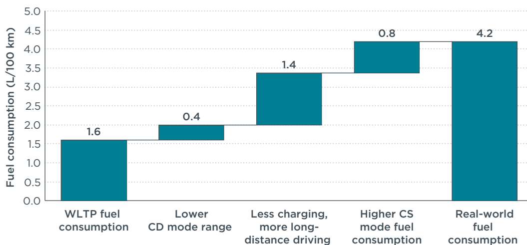
Figure 9. Contribution of different real-world factors to real-world fuel consumption of private car PHEVs.
