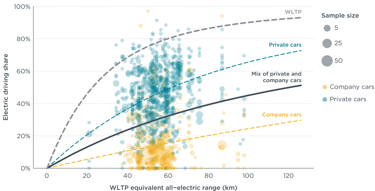
Figure 6. Real-world electric driving share of WLTP type-approved PHEVs compared to WLTP assumption on charge-depleting mode driving share and real-world adjusted UF curves.
