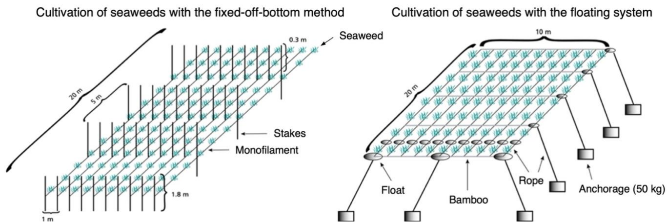
Fig. 1. Two primary methods for seaweed cultivation: fixed-off-bottom method and floating method. Dimensions, depths, materials, and anchorage weights will vary. Reproduced from Robledo et al. (2013) with permission.
