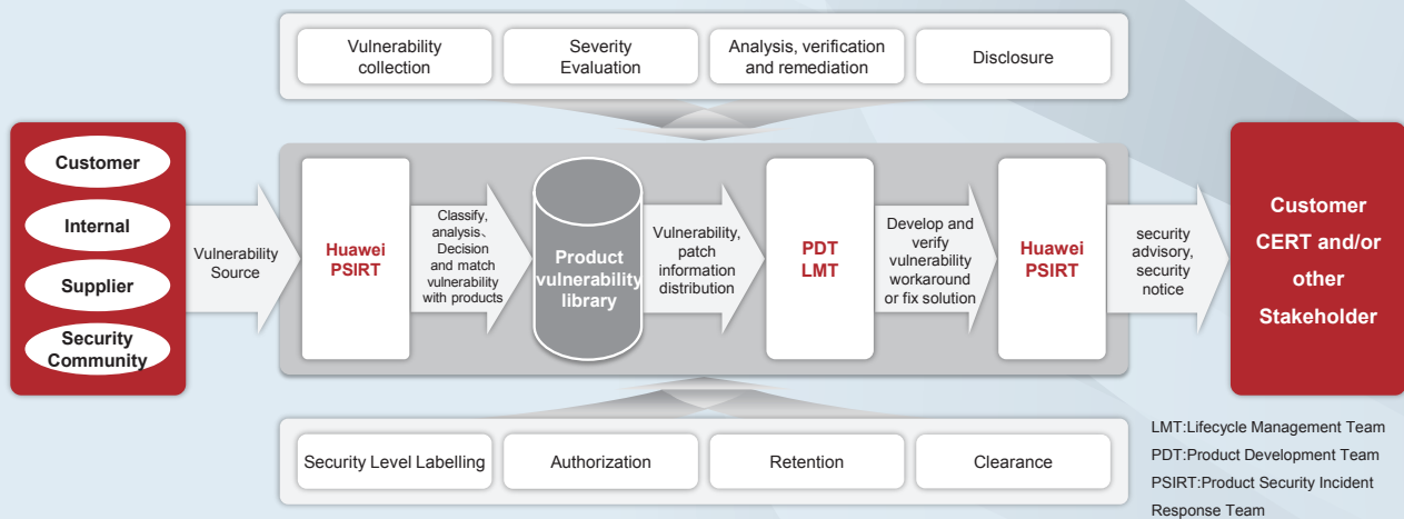
Figure 11, PSIRT/CERT process
