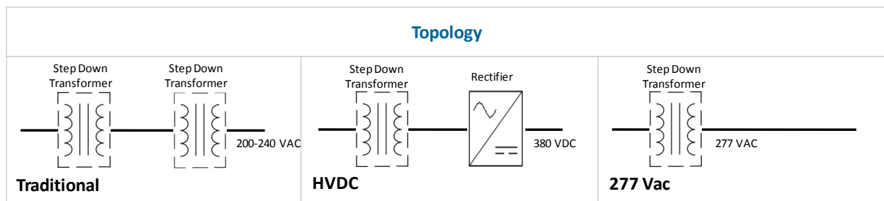
Figure 30 Most Common US Data Center Electrical Distribution Topologies
