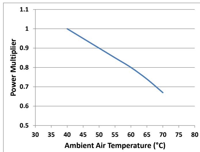
Figure 9 Example of power multipliers showing how power is de-rated (reduced) at ambient air temperatures above the full power capacity rating of 40°C (104°F).
