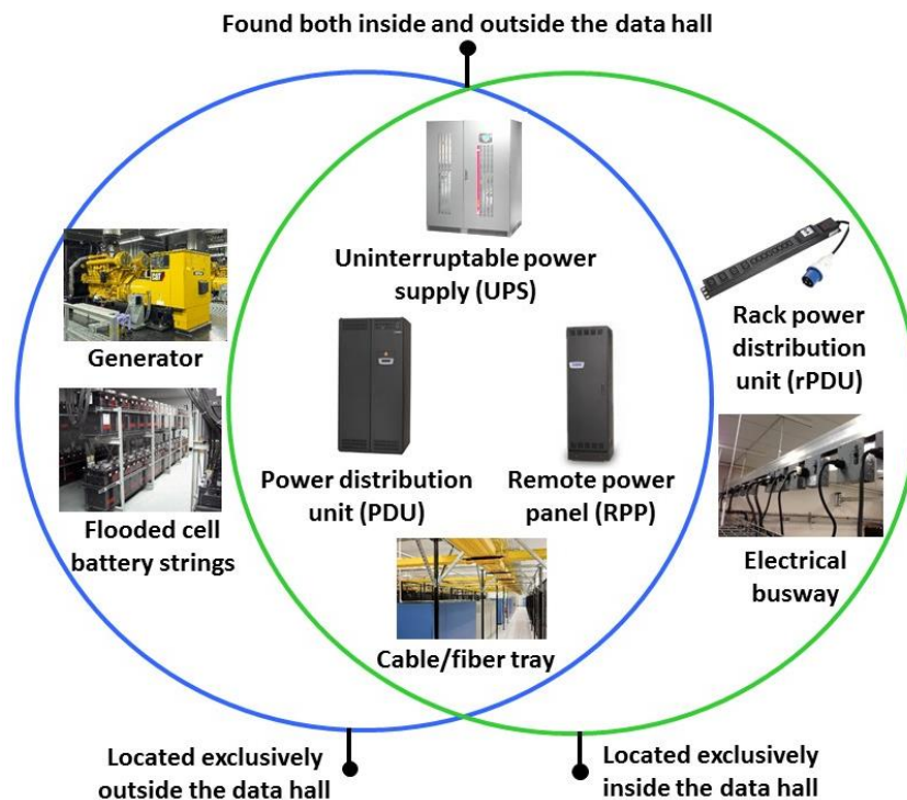
Figure 3 Venn diagram illustrating the physical location of data center power equipment.
