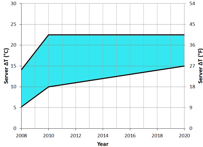
Figure 7 Server \Delta T projection at 35°C (95°F) server inlet temperature [15].
