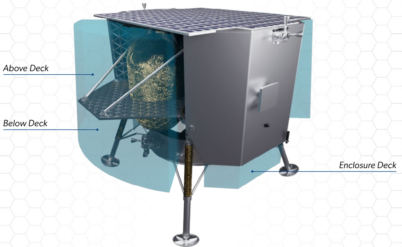
Peregrine - Standard Payload Mounting Envelopes
