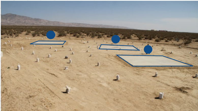
Early version of the OPAL sensor autonomously selects a hazard-free landing site for the Masten Space Systems Xombie Rocket.
