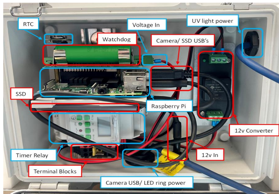
Figure 9: Annotated image of different components inside the AMI Connecting to the Pi
