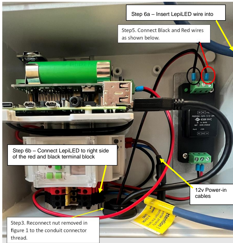
Figure 7: Wiring instructions
