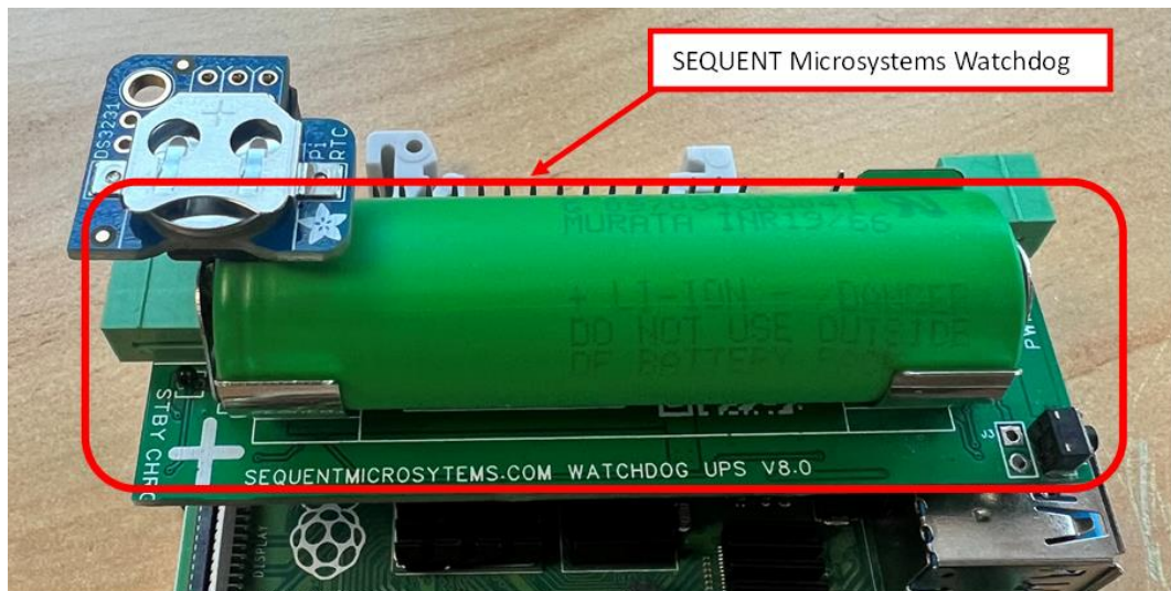
Figure 14: Image of the super watchdog-V8 with 18650 Battery installed
