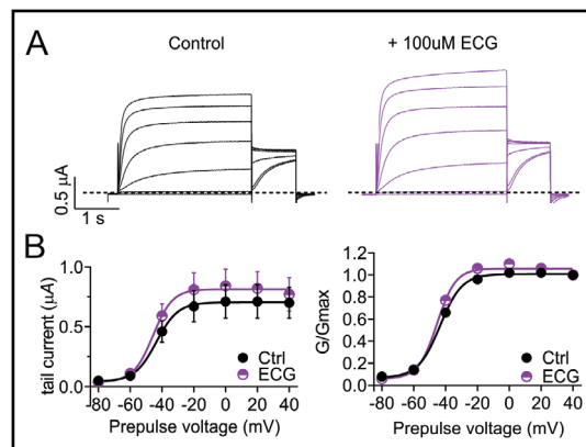
Fig. 6. Epicatechin gallate has negligible effects on KCNQ2/Q3. All error bars indicate SEM. A: Mean KCNQ2/Q3 traces in the absence (Control) and presence of 100 µM ECG (n = 5). B: Left, mean tail current; right, mean normalized tail current (G/Gmax) versus prepulse voltage for traces as in A (n = 5).
