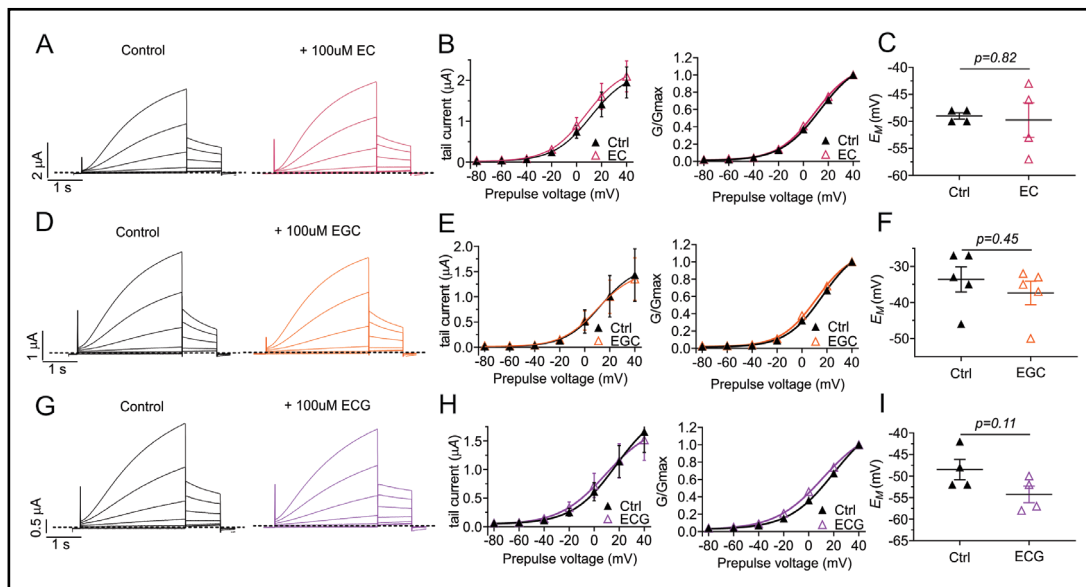
Fig. 5. EC, EGC and ECG have negligible effects on KCNQ1/E1 channels. All error bars indicate SEM. A: Mean KCNQ1/E1 traces in the absence (Control) and presence of 100 µM EC (n = 4). B: Left, mean tail current; right, mean normalized tail current (G/Gmax) versus prepulse voltage for traces as in A (n = 4). C: Scatter plot of unclamped membrane potential ( E_M ) for cells as in A (n = 4). Statistical analyses by two-way ANOVA. D: Mean KCNQ1/E1 traces in the absence and presence of 100 µM EGC (n = 5). E: Left, mean tail current; right, mean normalized tail current (G/Gmax) versus prepulse voltage for traces as in D (n = 5). F: Scatter plot of unclamped membrane potential ( E_M ) for cells as in D (n = 5). Statistical analyses by two-way ANOVA. G: Mean KCNQ1/E1 traces in the absence and presence of 100 µM ECG (n = 4). H: Left, mean tail current; right, mean normalized tail current (G/Gmax) versus prepulse voltage for traces as in G (n = 4). I: Scatter plot of unclamped membrane potential ( E_M ) for cells as in G (n = 4). Statistical analyses by two-way ANOVA.
