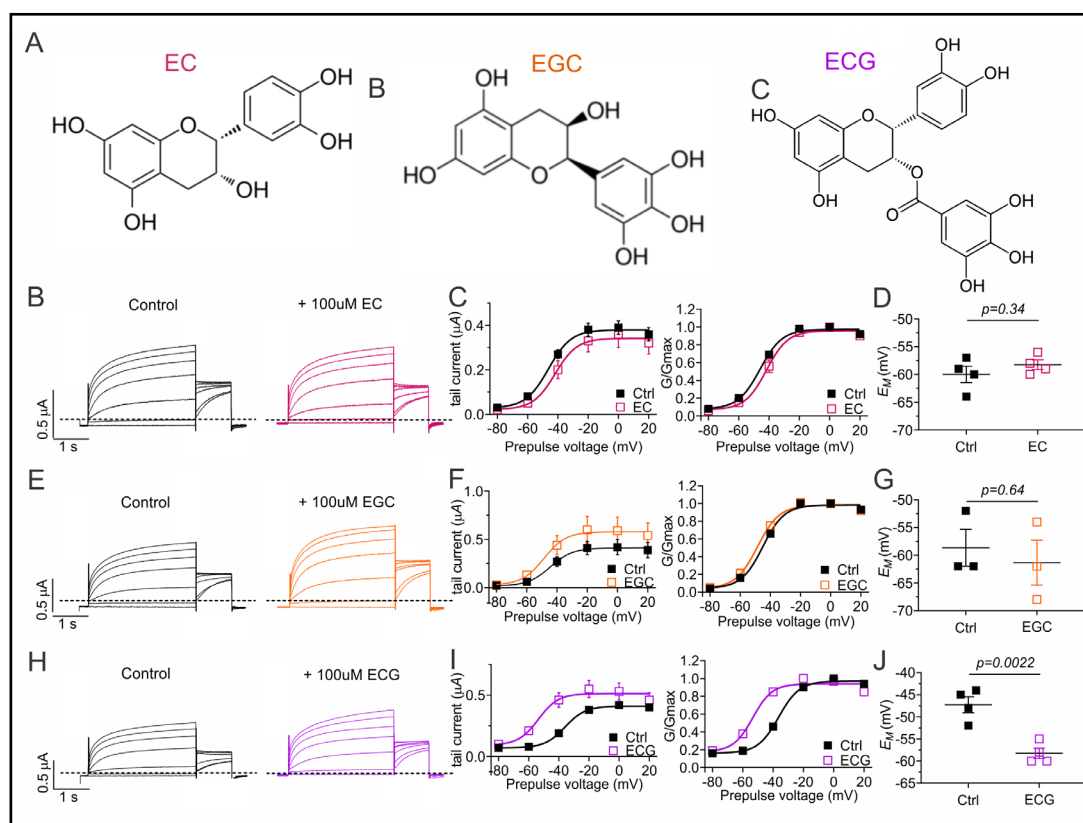
Fig. 4. Epicatechin gallate activates KCNQ5 channels. All error bars indicate SEM. A: Chemical structures of compounds used in this study, from left to right: (-)-epicatechin (EC), (-)-epigallocatechin (EGC), and (-)-epicatechin gallate (ECG). B: Mean KCNQ5 traces in the absence (Control) and presence of 100 \mu\text{M} EC ( n = 4 ). C: Left, mean tail current; right, mean normalized tail current ( G/G_{\text{max}} ) versus prepulse voltage for traces as in B ( n = 4 ). D: Scatter plot of unclamped membrane potential ( E_M ) for cells as in B ( n = 4 ). Statistical analyses by two-way ANOVA. E: Mean KCNQ5 traces in the absence (Control) and presence of 100 \mu\text{M} EGC ( n = 3 ). F: Left, mean tail current; right, mean normalized tail current ( G/G_{\text{max}} ) versus prepulse voltage for traces as in E ( n = 3 ). G: Scatter plot of unclamped membrane potential ( E_M ) for cells as in E ( n = 3 ). Statistical analyses by two-way ANOVA. H: Mean KCNQ5 traces in the absence (Control) and presence of 100 \mu\text{M} ECG ( n = 4 ). I: Left, mean tail current; right, mean normalized tail current ( G/G_{\text{max}} ) versus prepulse voltage for traces as in H ( n = 4 ). J: Scatter plot of unclamped membrane potential ( E_M ) for cells as in H ( n = 4 ). Statistical analyses by two-way ANOVA.
