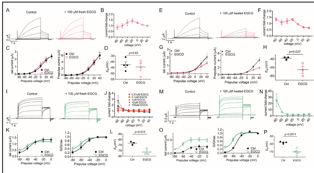
Fig. 8. Heating EGCG enables KCNQ1/E1 inhibition and KCNQ5 activation. All error bars indicate SEM. A: Mean KCNQ1/E1 traces in the absence (Control) and presence of 100 \mu\text{M} fresh EGCG (n = 4). B: KCNQ1/E1 tail current fold-change versus voltage for traces as in A (n = 4). C: Left, mean tail current; right, mean prepulse current versus prepulse voltage for traces as in A (n = 4). D: Scatter plot of unclamped membrane potential ( E_M ) for cells as in A (n = 4). Statistical analyses by two-way ANOVA. E: Mean KCNQ1/E1 traces in the absence (Control) and presence of 100 \mu\text{M} heated EGCG (n = 4). F: KCNQ1/E1 tail current fold-change versus voltage for traces as in E (n = 4). G: Left, mean tail current; right, mean prepulse current versus prepulse voltage for traces as in E (n = 4). H: Scatter plot of unclamped membrane potential ( E_M ) for cells as in E (n = 4). Statistical analyses by two-way ANOVA. I: Mean KCNQ5 traces in the absence (Control) and presence of 100 \mu\text{M} fresh EGCG (n = 4). J: KCNQ5 tail current fold-change versus voltage for traces as in I, for a range of fresh EGCG concentrations (n = 4). K: Left, mean tail current; right, mean normalized tail current (G/Gmax) versus prepulse voltage for traces as in I (n = 4). L: Scatter plot of unclamped membrane potential ( E_M ) for cells as in I (n = 4). Statistical analyses by two-way ANOVA. M: Mean KCNQ5 traces in the absence (Control) and presence of 100 \mu\text{M} heated EGCG (n = 4). N: KCNQ5 tail current fold-change versus voltage for traces as in M (n = 4). O: Left, mean tail current; right, mean normalized tail current (G/Gmax) versus prepulse voltage for traces as in M (n = 4). P: Scatter plot of unclamped membrane potential ( E_M ) for cells as in M (n = 4). Statistical analyses by two-way ANOVA.
