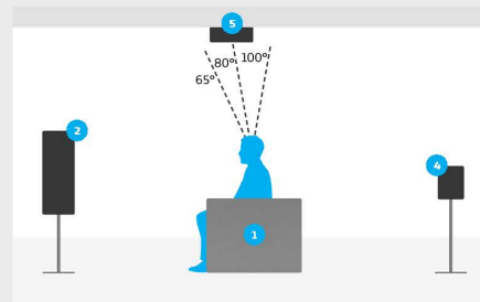
Overhead speaker placement detail for 4.1.2 setup
