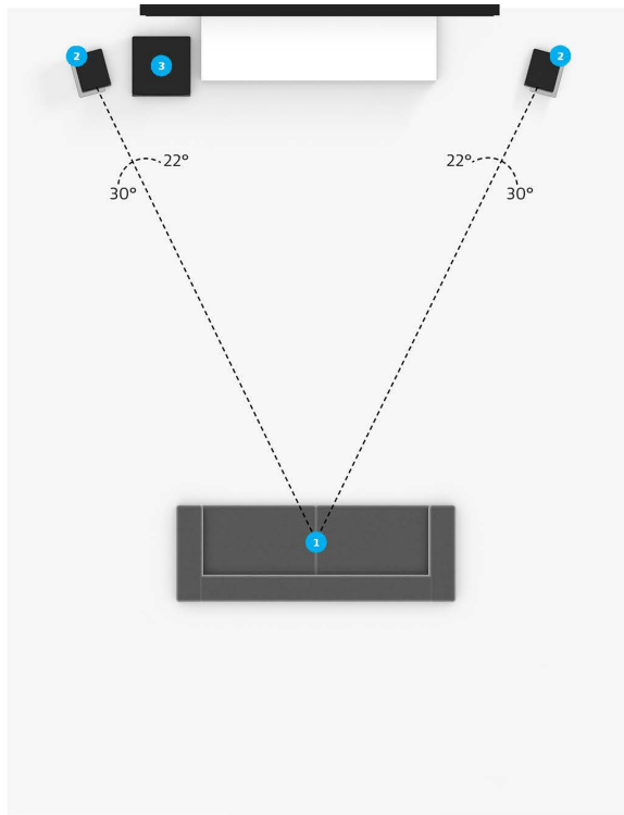
Speaker placement for 2.1 setup
