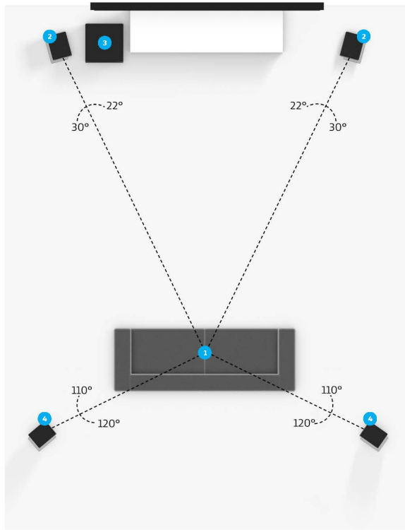
Speaker placement for 4.1 setup
