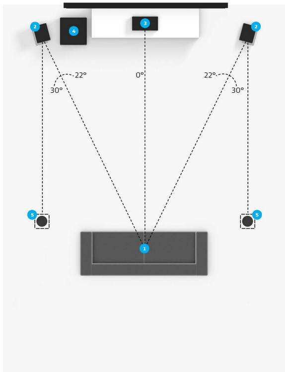
Speaker placement for 3.1.2 setup
