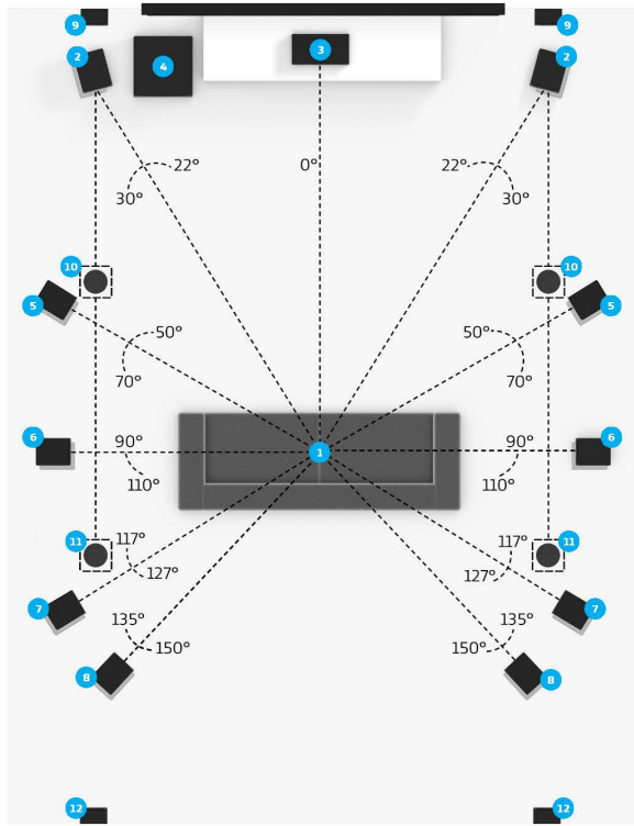
Speaker placement for 11.1.8 setup
