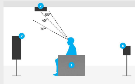
Overhead speaker placement detail for 7.1.6 hybrid setup
