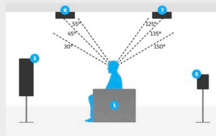
Overhead speaker placement detail for 5.1.4 setup
