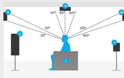
Overhead speaker placement detail for 9.1.6 setup
