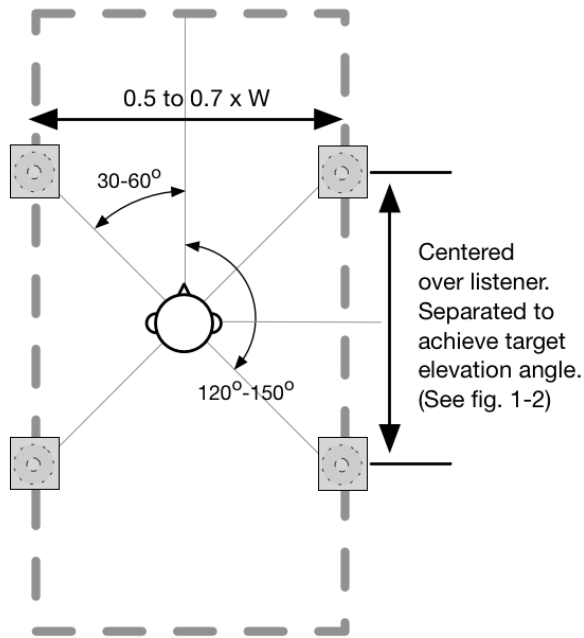
Figure 4: Top view, height (overhead) speaker positioning.
