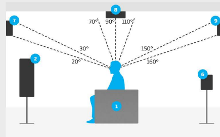
Overhead speaker placement detail for 7.1.6 setup
