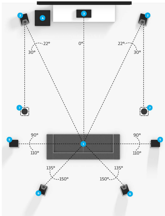
Speaker placement for 7.1.6 setup
