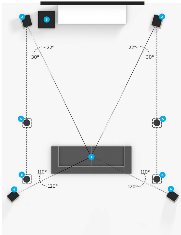
Speaker placement for 4.1.4 setup
