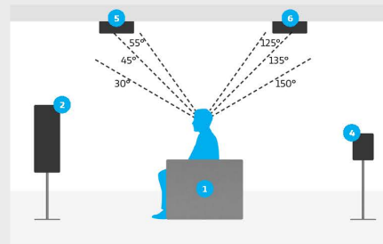
Overhead speaker placement detail for 4.1.4 setup
