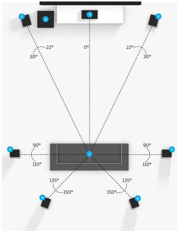
Speaker placement for 7.1 setup
