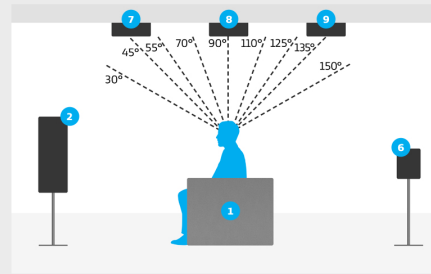
Overhead speaker placement detail for 7.1.6 setup
