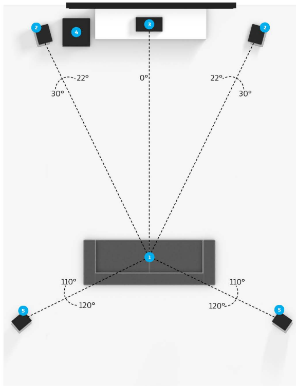
Speaker placement for 5.1 setup
