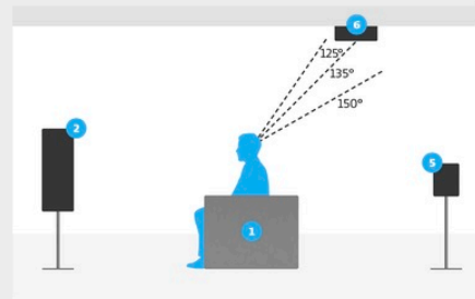
Overhead speaker placement detail for 5.1.4 hybrid setup
