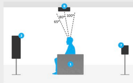
Overhead speaker placement detail for 9.1.2 setup
