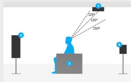
Overhead speaker placement detail for 7.1.4 hybrid setup
