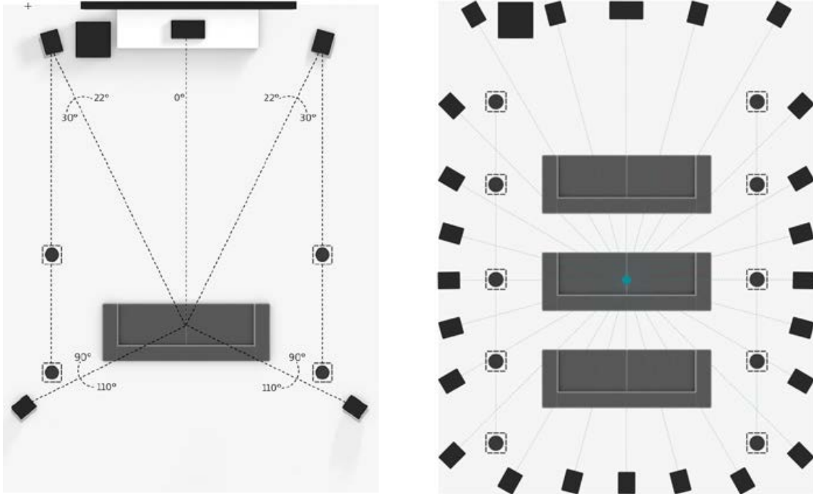
Figure 1: At left is a Dolby Atmos system with five speakers on the floor and four overhead speakers; at right is a Dolby Atmos system with up to 24 speakers on the floor and 10 overhead speakers.
