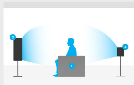
Virtual speaker placement: detail for 4.1 setup
