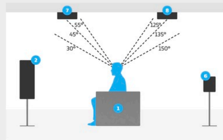
Overhead speaker placement detail for 7.1.4 setup
