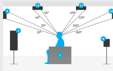
Overhead speaker placement detail for 11.1.8 setup
