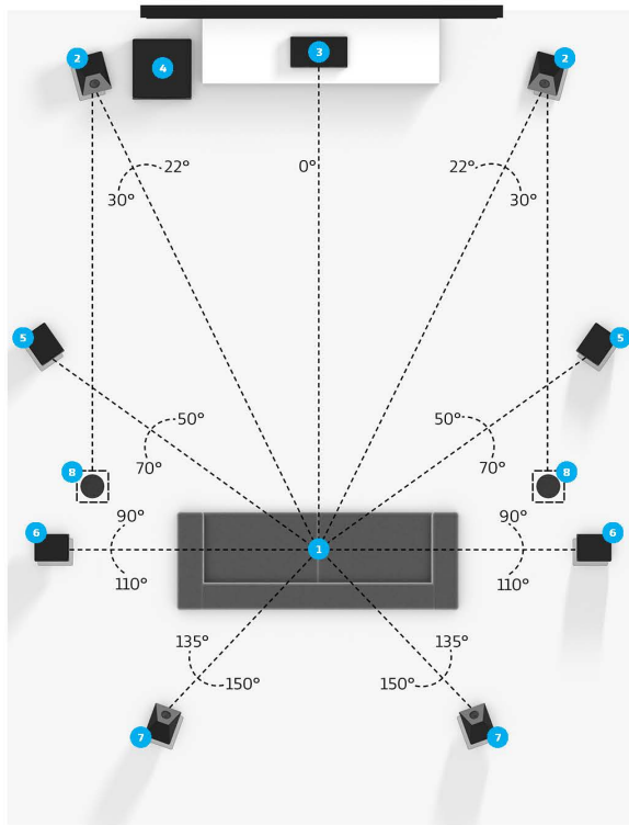
Speaker placement for 9.1.6 setup
