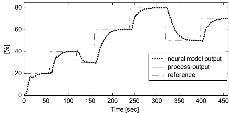
Figure 3: Process neural model validation
