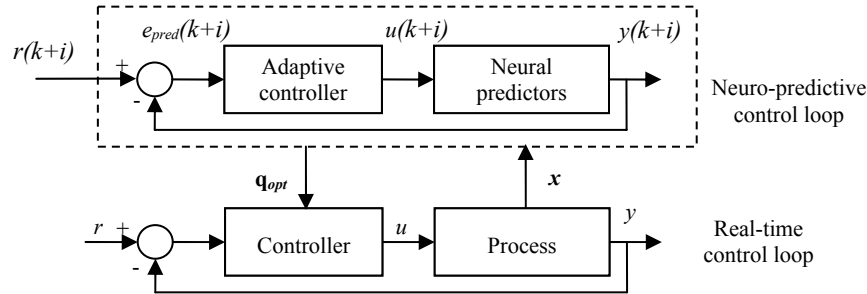
Figure 1: Neuro-predictive structure
