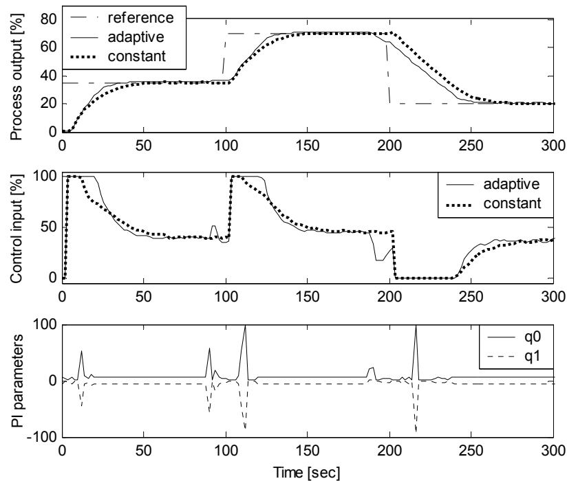
Figure 4: Comparative results and parameters for the adaptive discrete PI controller
