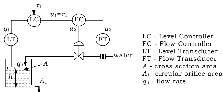
Figure 2: Schematic diagram of the level-flow pilot plant
