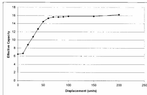
Fig. 4: Effective Capacity vs displacement for a locally-connected network of 500 units, each with 50 afferent connections. Results are averages over 200 runs.
