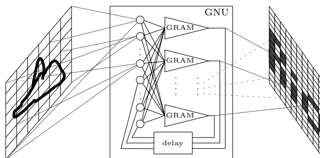
Fig. 2: GNU architecture
