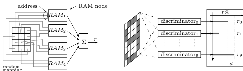
Fig. 1 – Example of a RAM-discriminator and of a WiSARD
