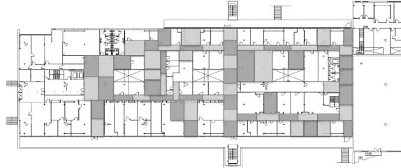
Fig. 3: Institute floor plan
