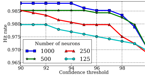
Fig. 6: Experiment 1 results. Observations size: 100 \times 124 pixels \Rightarrow Input size: 12400 bits. 1000 neurons \Rightarrow 13-tuple nodes; ... 125 neurons \Rightarrow 100-tuple nodes.
