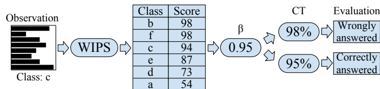
Fig. 5: To evaluate WIPS, an observation whose real class, c , is known is input as a query. A rank of all classes and their respective scores is output. Class c score divided by the highest score is \beta = 94/98 \simeq 0.95 . Iff \beta \geq CT , the output is accepted as correct.
