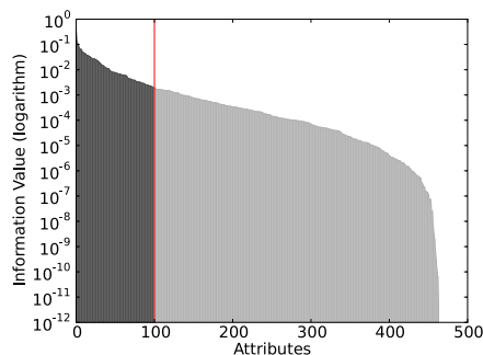
Fig. 2: Information value of the attributes.
