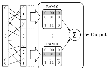
Fig. 1: Example of access in a discriminator.
