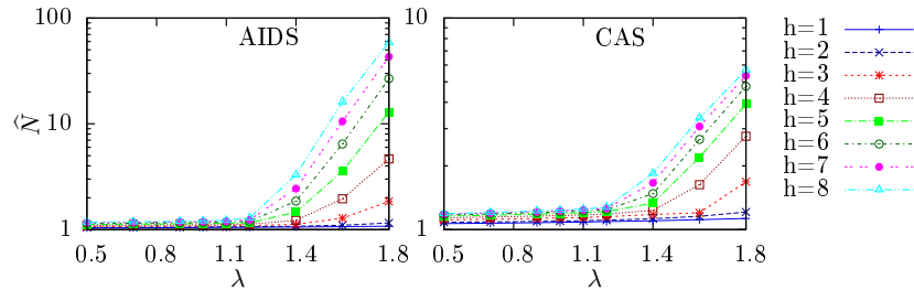
Fig. 3: \widehat{N} of the ODD_{ST} kernel for different values of h and \lambda , and datasets.
