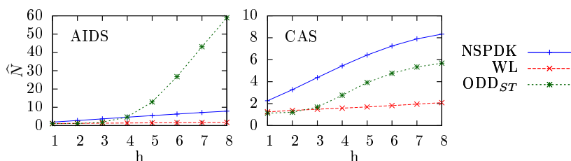
Fig. 1: \hat{N} as a function of the h parameter for kernels and datasets.
