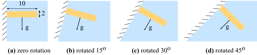
Figure 2.16: Setup of the 2D cantilever problem under different rotation angles. (a) 0^\circ , (b) 15^\circ , (c) 30^\circ , and (d) 45^\circ .
