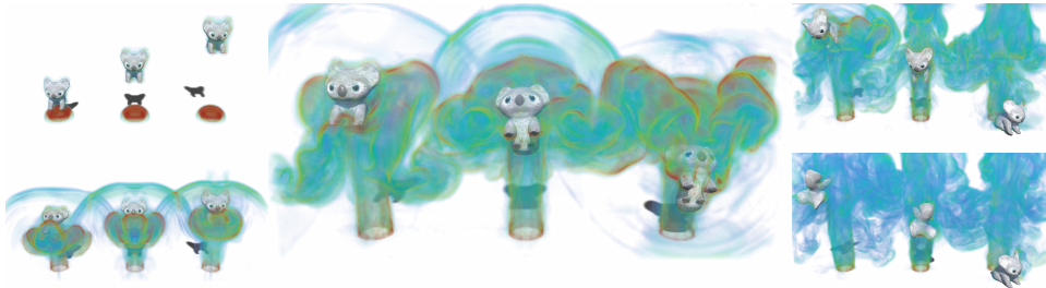
Figure 3.19: Demo: Three koala toys hit by Mach diamond jets. The inlet setting mimics the 2D version in Figure 3.18. The density ratio (from left to right) of the koalas is 1:4:9. The lightest koala is easily propelled upward; the middle one maintains balance under the effects of the pumping jet and gravity; the heaviest koala easily disrupts the jet's wavefront.
