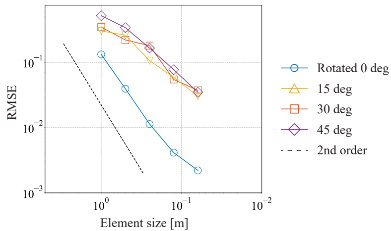
Figure 2.19: Convergence plot of the displacements of the 2D cantilever with rotations.
