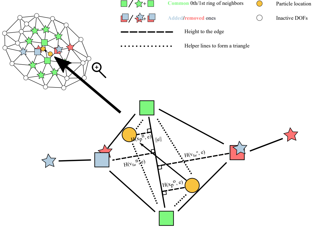
Figure 2.3: A visual proof that \eta diminishes locally. As described in (2.31), for every vertex v within the first ring of neighbors, \mathcal{N}_{a,r}^1 . The dashed line denotes the perpendicular height from a given position to the shared edge. Dotted lines are drawn to construct a triangle between the point \mathbf{x}_p and the edge, facilitating the computation of the barycentric coordinates.
