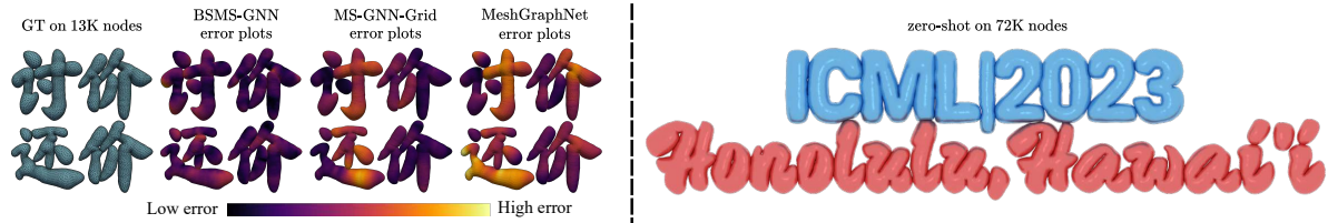
Figure 4.7: Zero-shot ability of BSMS-GNN. Left: Comparing the rollout RMSE between BSMS-GNN and existing SOTAs on the INFLATINGFONT benchmark. Our framework reaches the highest accuracy, demonstrating a stronger capability for complex, large geometries with massive contacts. Right: Our trained model can zero-shot infer on never-seen fonts, with about 7\times more nodes in the mesh size while maintaining the same accuracy.
