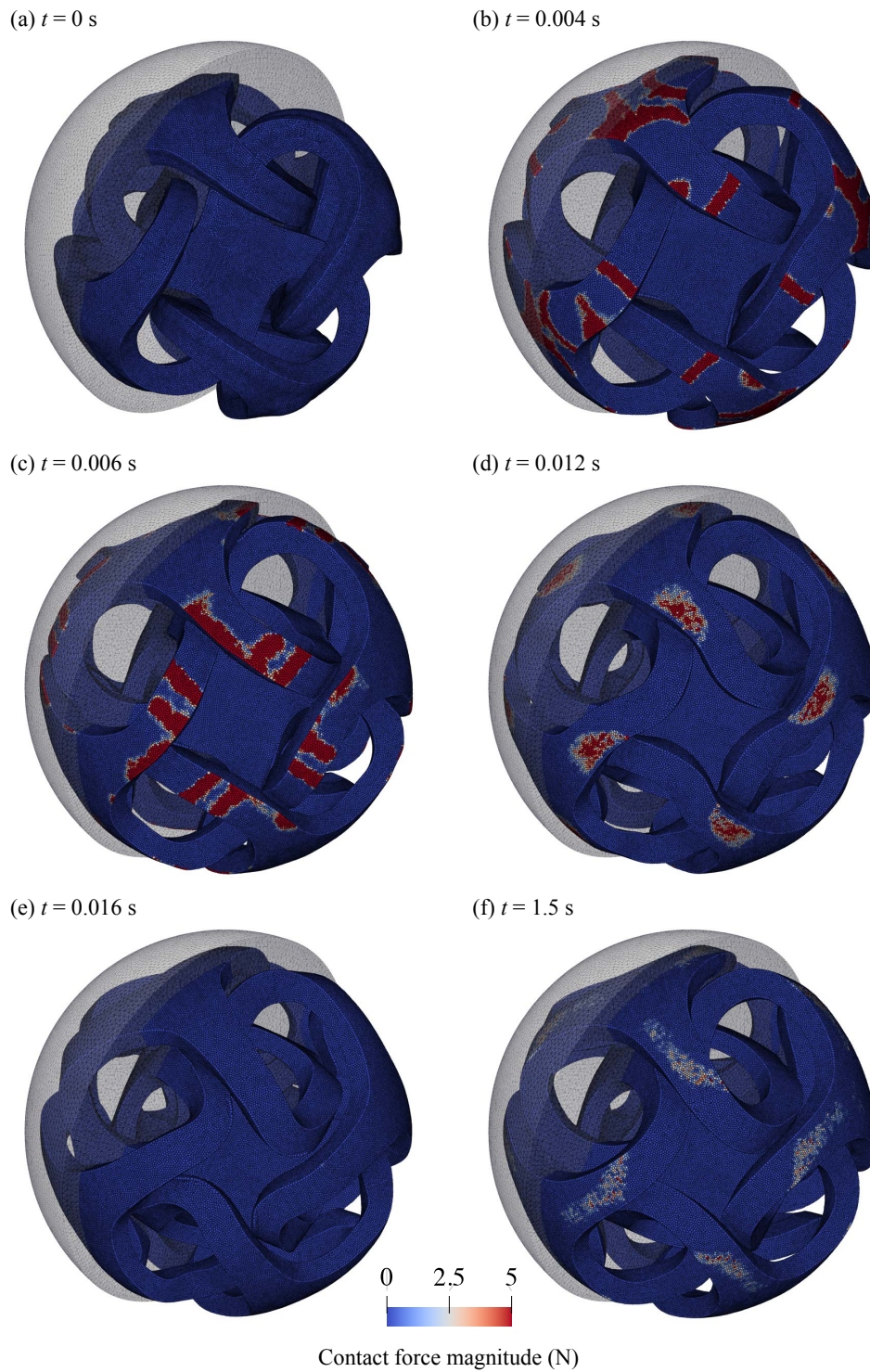
Figure 2.25: The contact force magnitude of the 3D elastic object expansion.
