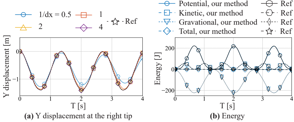
Figure 2.17: Displacements and system energy of the 2D cantilever without rotation. Plots of (a) the displacement in the y -direction at the right tip of the cantilever and (b) the energies of the system.
