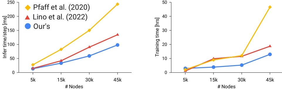
Figure 4.10: Scaling analysis for different baselines. As the size of the font dataset (INFLATINGFONT) increases, our proposed method (BSMS-GNN) consistently outperforms both MESHGRAPHNETS and MS-GNN-GRID in terms of efficiency and scalability.
