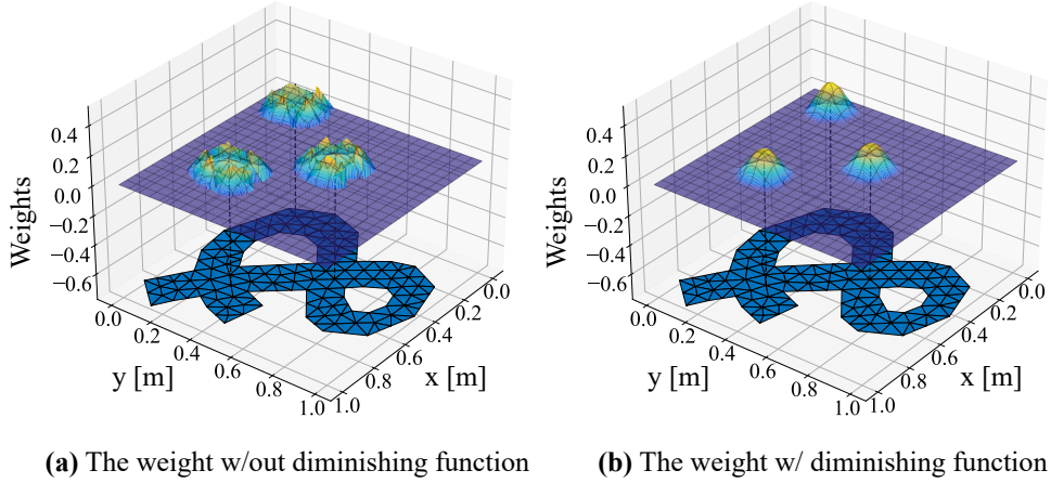
Figure 2.8: Ablation study of reconstruction with or without diminishing on 2D mesh. (a) without and (b) with the application of the diminishing function.
