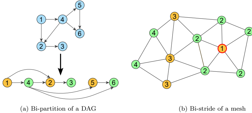
Figure 4.1: Similarity between Bi-partition and Bi-stride. The number in the circle indicates the depth of the frontiers of topological sorting or BFS. The red-bordered circle (number 1) represents the starting node, i.e., the seed.
