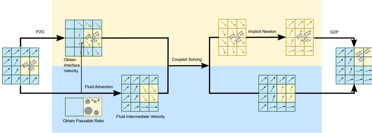
Figure 3.1: Algorithm overview for CSMPM. This schematic illustrates our method. The pipeline commences with previously advected particles transferring their physical properties to a background grid through a Particle-to-Grid (P2G) process. The grid is employed for: a) implicit integration of the solids (upper row), and b) estimating a passable ratio for more accurate flow advection (bottom row). Based on degrees-of-freedom (DOFs) on the grid, we assemble and solve a coupled velocity-pressure system to advance these quantities to the next step. Section 2.2 presents a more detailed overview of our full algorithm.
