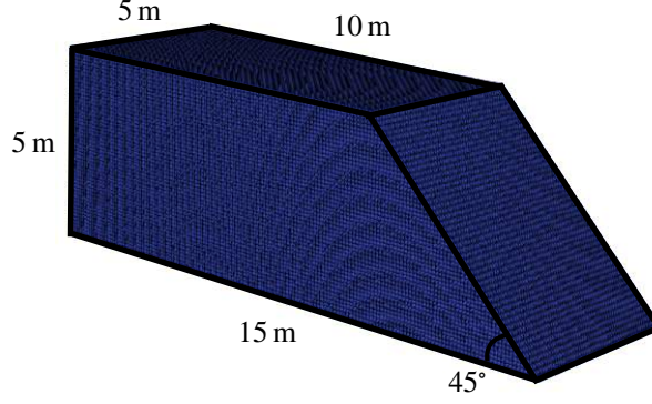
Figure 2.20: Setup of the 3D slope failure. Geometry adapted from (Zhao et al., 2023b).
