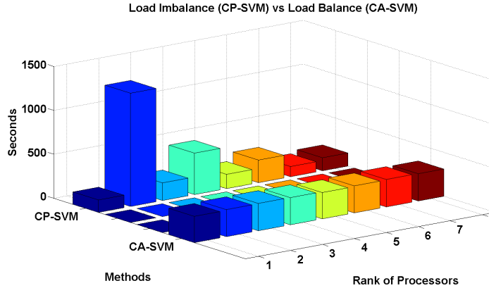
Figure 2.6: The figure shows that CP-SVM is load imbalanced while CA-SVM is load-balanced. The test dataset is epsilon with 128,000 samples (2,000 nnz per sample). 8 nodes are used in this test.
