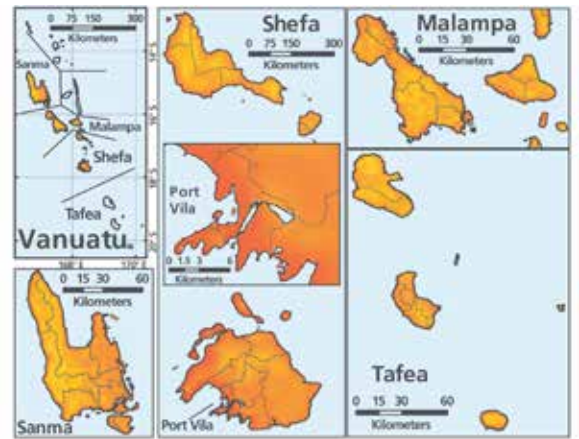
Figure 5 — Peak horizontal acceleration of the ground (Note: 1g is equal to the acceleration of gravity) that has about a 40% chance to be exceeded at least once in the next 50 years.
