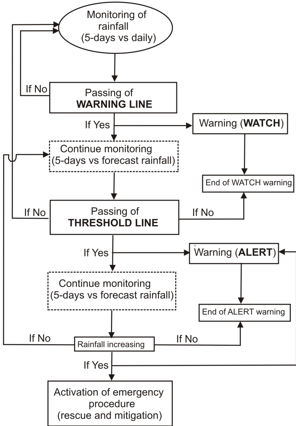
Figure 1 Operating procedure of warning system based on rainfall thresholds.
