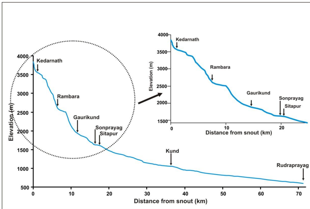
(Fig. 1. Longitudinal profile of Mandakini river showing distinct slope breaks around Kedarnath, Rambara and Sonprayag-Sitapur (inset: section enlarged between Kedarnath and Sitapur). These discontinuities acted as depocenters for the sediments transported down valley from Kedarnath).
