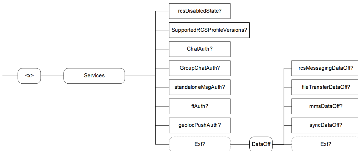
Figure 22: RCS additions, Services sub tree
