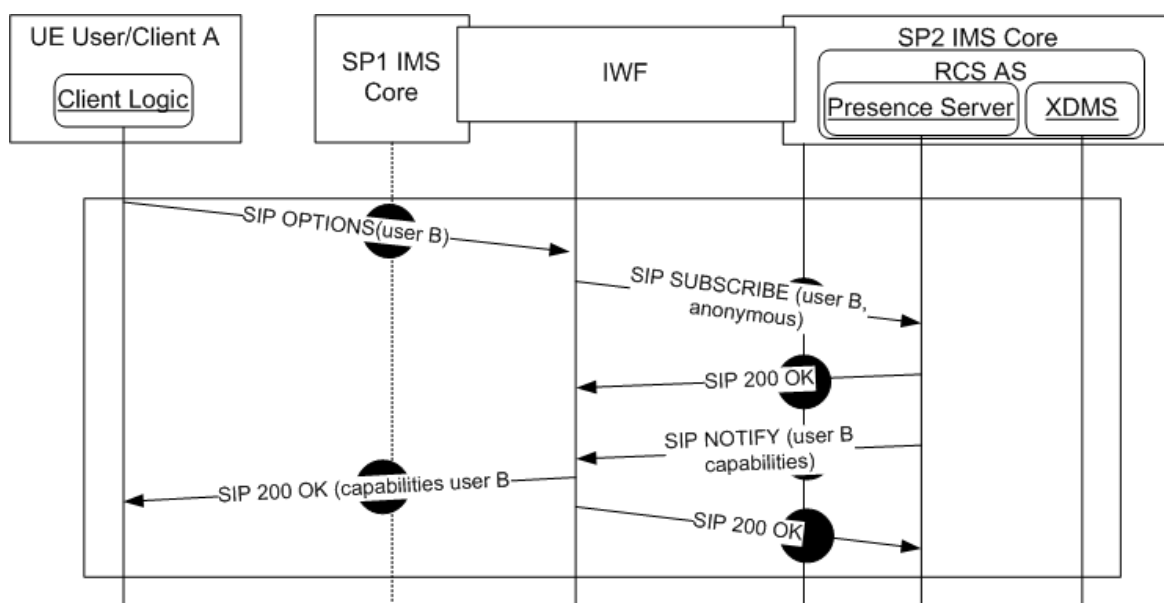
Figure 4: Capability interworking via network: Options request
