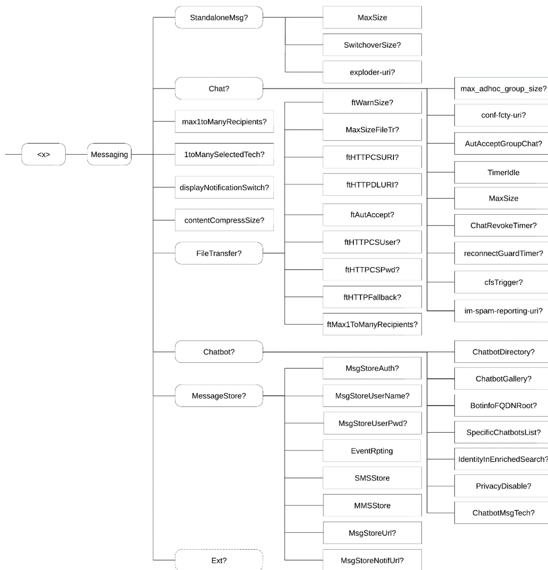
Figure 23: RCS additions to the IM MO sub tree
