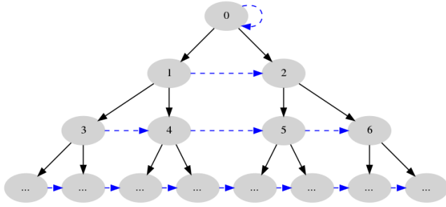
Figure 1: Complex decomposition of \mathcal{T} via task partitioning for a single robot. \mathcal{G}_d(\mathcal{V}_a, \mathcal{E}_d) is a complete binary tree formed by the black edges connecting the task nodes. Each \phi_i is formed by connecting the nodes at height i within \mathcal{G}_d(\mathcal{V}_a, \mathcal{E}_d) together with the blue edges.
