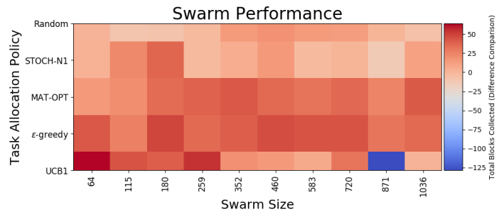
Figure 9: Performance difference comparison on a compound task decomposition graph between swarms operating under matroid optimality constraints vs. relaxation. Negative values indicate that a performance drop was observed when constraints were relaxed, when compared with Fig. 8.
