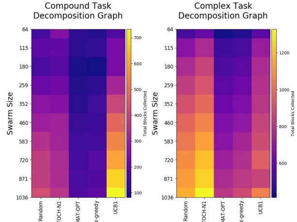
Figure 8: Performance for all methods on compound and complex task decomposition graphs scenario in Fig. 6 using a 10% swarm density under imperfect information.
