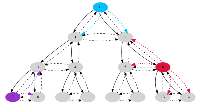
Figure 2: Task allocation neighborhoods \mathcal{G}_{nbhd}(\mathcal{V}_{nbhd}, \mathcal{E}_{nbhd}) within \mathcal{G}_a(\mathcal{V}_a, \mathcal{E}_a) induced by \mathcal{E}_{nbhd} for each v_f \in \mathcal{V}_a . A task is either the root (node 0, blue), a leaf node (node 7, purple), or neither (node 6, red). The three possible cases of allocation neighborhoods reachable from v_f are shown via different colored edges.
