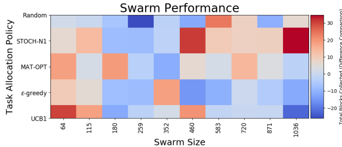
Figure 10: Performance difference comparison on a complex task decomposition graph between swarms operating under matroid optimality constraints vs. relaxation. Negative values indicate that a performance drop was observed when constraints were relaxed, when compared with Fig. 8.
