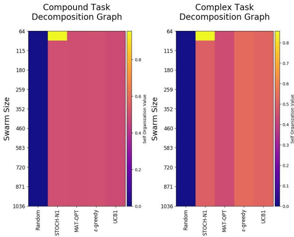
Figure 7: Observed emergent intelligence via self-organization for all methods on compound and complex task decomposition graph for scenario in Fig. 6 using a 10% swarm density under imperfect information.
