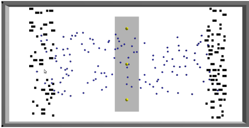
Figure 6: Screen shot of a dual source foraging scenario with multiple robots (blue blobs), objects to be collected (black squares), and the nest in the center (gray).
