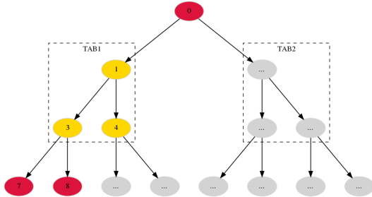
Figure 4: Task Allocation Contexts (TABs) within \mathcal{G}_a(\mathcal{V}_a, \mathcal{E}_a) . v_f with unambiguous partition points in red (root and leaf nodes), and ambiguous partition points in gold.
