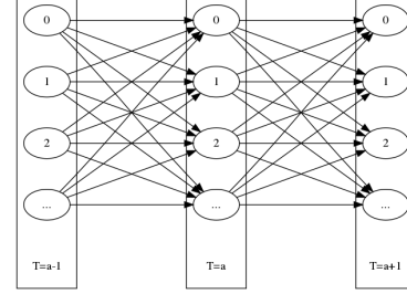
Figure 3: Unrolled task allocation graph \mathcal{G}_{|A|}(\mathcal{V}_{|A|}, \mathcal{E}_{|A|}) shown for arbitrary task allocation times a - 1, a, a + 1 .
