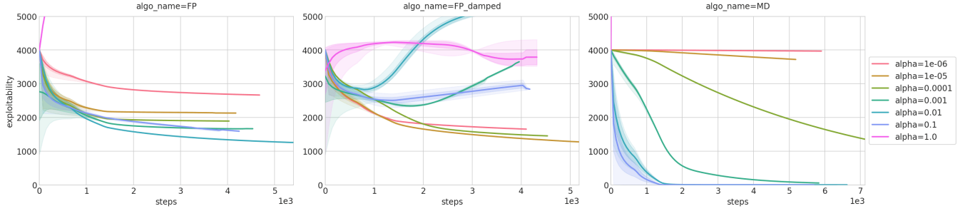
Figure 1: 5 Garnet sampled with param n_x = 20000 , n_a = 10 , t = 2000 , s_f = 10
