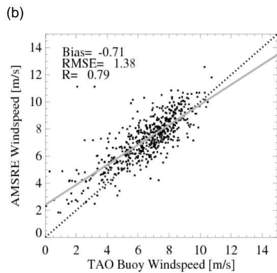
Figure 2: Scatterplot (a) between the TAO WS and the HS WS, (b) between the TAO WS and the WS provided by the current AMSR-E WS.
