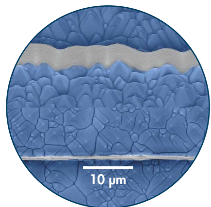
High AR silver line on solar cell
