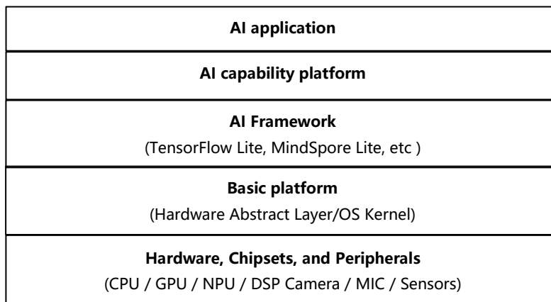
Figure 3: AI Architecture
