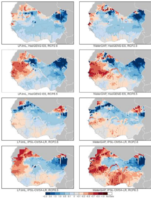
Figure 41: ISIMIP Average Index Values against 1970–2010 Baseline for Water Availability, West Africa, 2050–2100. Note: Data compiled from LPJmL/water (panel a) and WaterGAP (panel b), forced with the HadGEM2-ES climate model (top four maps) and IPSL-CM5A (bottom four maps) under RCP2.6 and RCP8.5. Blue areas indicate wetting relative to the historical baseline, and gray and tan areas indicate drying.
