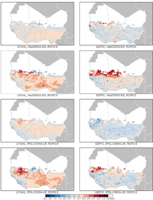
Figure 42: ISIMIP Average Index Values against 1970–2010 Baseline for Crop Production, West Africa, 2050–2100. Note: Data compiled from LPJmL/crop (panel a) and GEPIC (panel b), forced with the HadGEM2-ES climate model (top four maps) and IPSL-CM5A (bottom four maps) under RCP2.6 and RCP8.5. Blue areas indicate wetting relative to the historical baseline, and tan to red areas indicate drying. White areas do not grow the four major crops.
