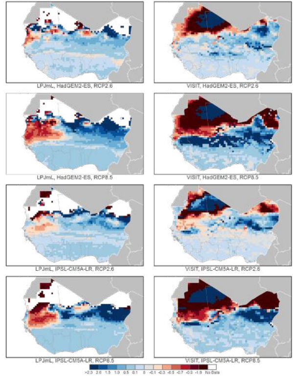
Figure 43: ISIMIP Average Index Values against 1970–2010 Baseline for Ecosystem NPP, West Africa, 2050–2100. Note: Data compiled from LPJmL (panel a) and VISIT (panel b), forced with the HadGEM2-ES climate model (top four maps) and IPSL-CM5A (bottom four maps) under RCP2.6 and RCP8.5. Blue areas indicate higher NPP relative to the historical baseline, and tan to red areas indicate lower NPP. NPP = net primary productivity.
