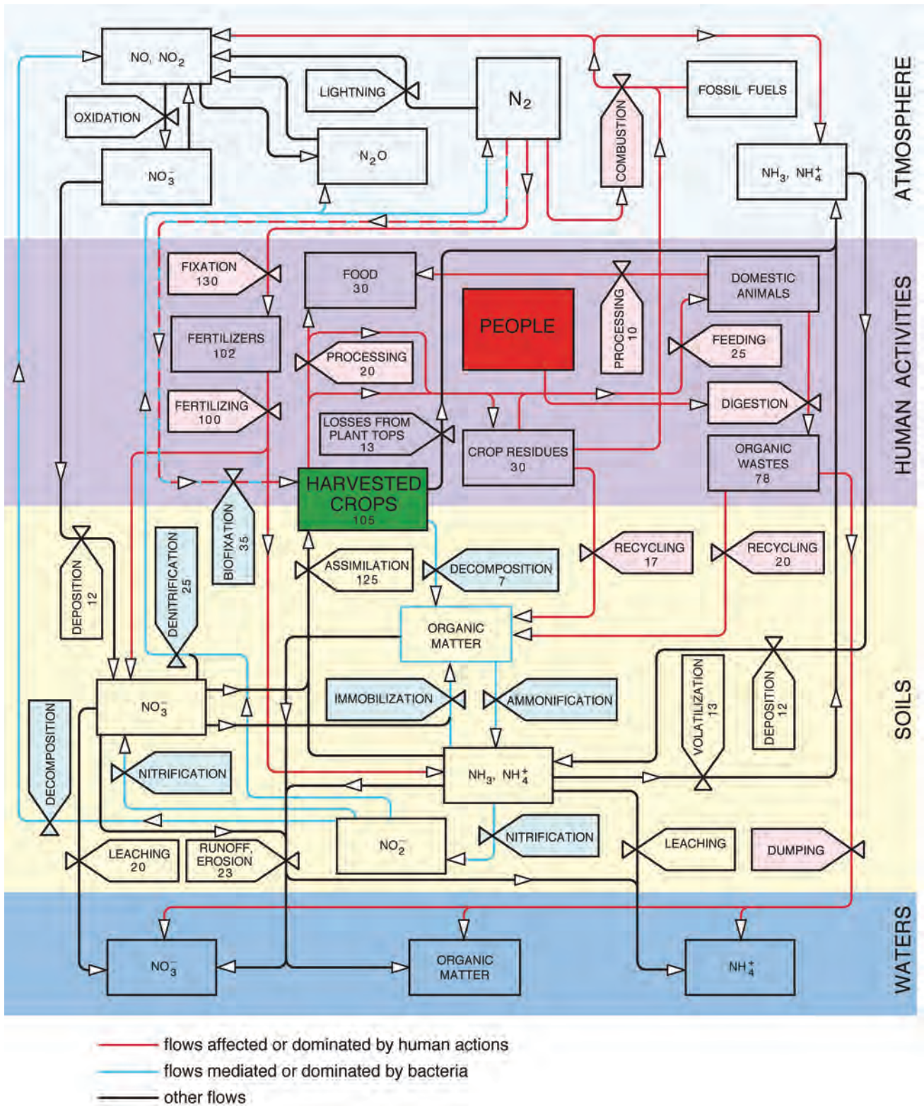
Fig 1 Nitrogen cycling in the global agroecosystem. Stores are shown as rectangles and flows as valves. The cycle is subdivided into its three principal environmental compartments (atmosphere, soils and waters) and all flows affected or dominated by human actions (and hence the targets of possible efficiency improvements) are shown in red while the flows mediated or dominated by bacterial metabolism are in blue. The latest available crop production, livestock and fertilizer statistics from FAO and IFA and nitrogen contents from Smil (2001) were used to calculate the stores and flows as annual averages for the period 2005-2009. Their accuracy varies from high (fertilizers, food) to poor (runoff, denitrification). Food (30 Mt N) corresponds to average global per capita daily intakes of 50 g of plant and 25 g of animal protein (excluding aquatic species). The difference between fixation and fertilizers is ammonia used as feedstock in chemical syntheses.
