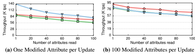
Figure 15: Attributes Accessed – Evaluation of the version storage schemes using YCSB ( \theta=0.2 ) with 40 DBMS threads and varying the number of the tuples’ attributes that are accessed per read operation.
