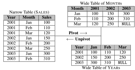
Figure 4: Pivot table example, reproduced from [27], demonstrating pivoting over two separate columns, “Month” and “Year”.
