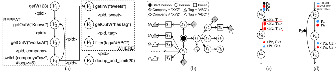
Figure 1: (a) The logical dataflow for Example 1. (b) An example data graph. (c)(d) Execution pipelines illustrating how the where and repeat subquery in Figure 1(a) process the example data graph in topo-static dataflow model. For simplicity, the execution pipelines only depict a snippet of messages generated during query execution.
