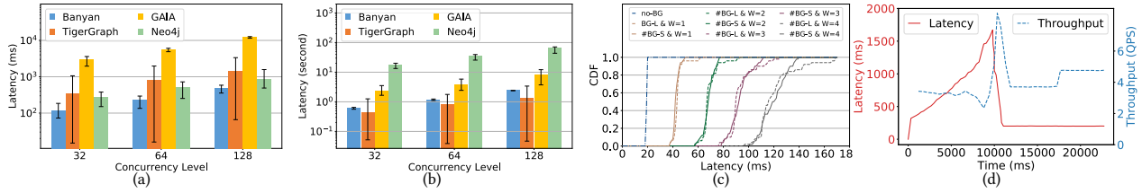
Figure 7: The latency of Banyan, TigerGraph, GAIA and Neo4j under different concurrent workloads: (a) the latency of small queries and (b) the latency of large queries. (c) The latency CDF of the foreground query under different background workloads. (d) The throughput and latency of Banyan before and after load balancing.
