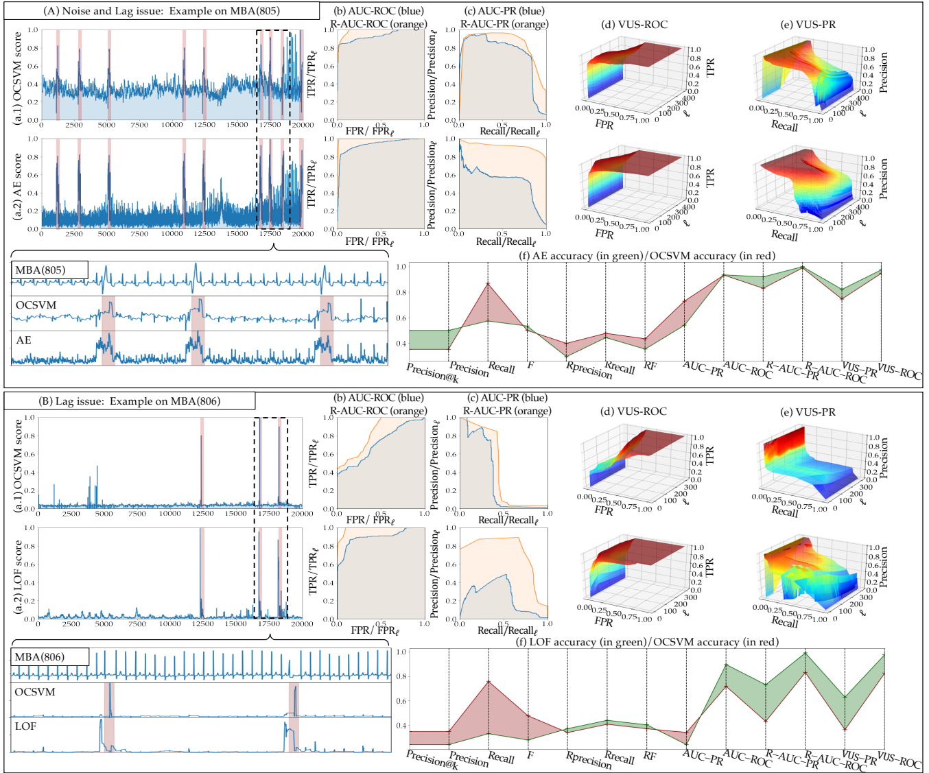
Figure 5: Comparison of evaluation measures (proposed measures illustrated in subplots (b,c,d,e); all other measures summarized in subplots (f)) on two examples ((A) AE and OCSM applied on MBA(805) and (B) LOF and OCSVM applied on MBA(806)), illustrating the limitations of existing measures when the anomaly score or label is either noisy or lagged, due to labeling errors (or different labeling conventions).
