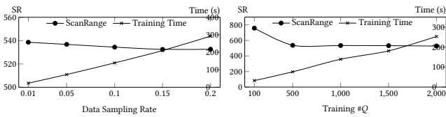
Figure 12: Varying data sampling size.
