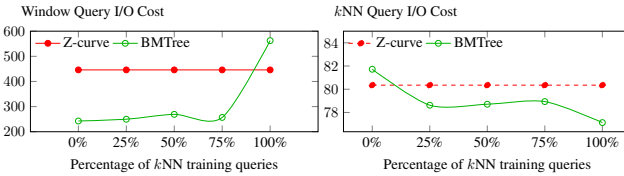
(a) Window Query I/O
