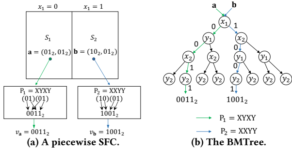
Figure 4: (a) An example of a piecewise SFC, which comprises two BMPs P_1 and P_2 for computing values of data points a and b. (b) A BMTree that combines the two BMPs.
