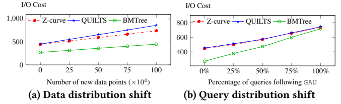
Figure 14: Performance under data & query distribution shift.
