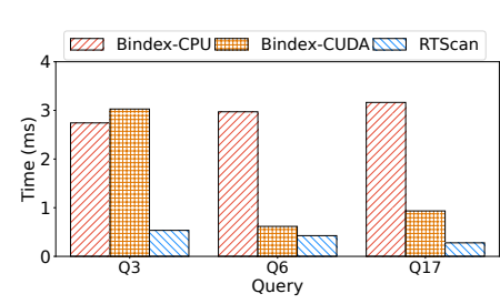
Figure 21: Performance of RTScan with TPC-H dataset
