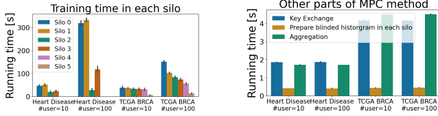
Figure 10: With a small model, the private weighting protocol has a practical execution time.
