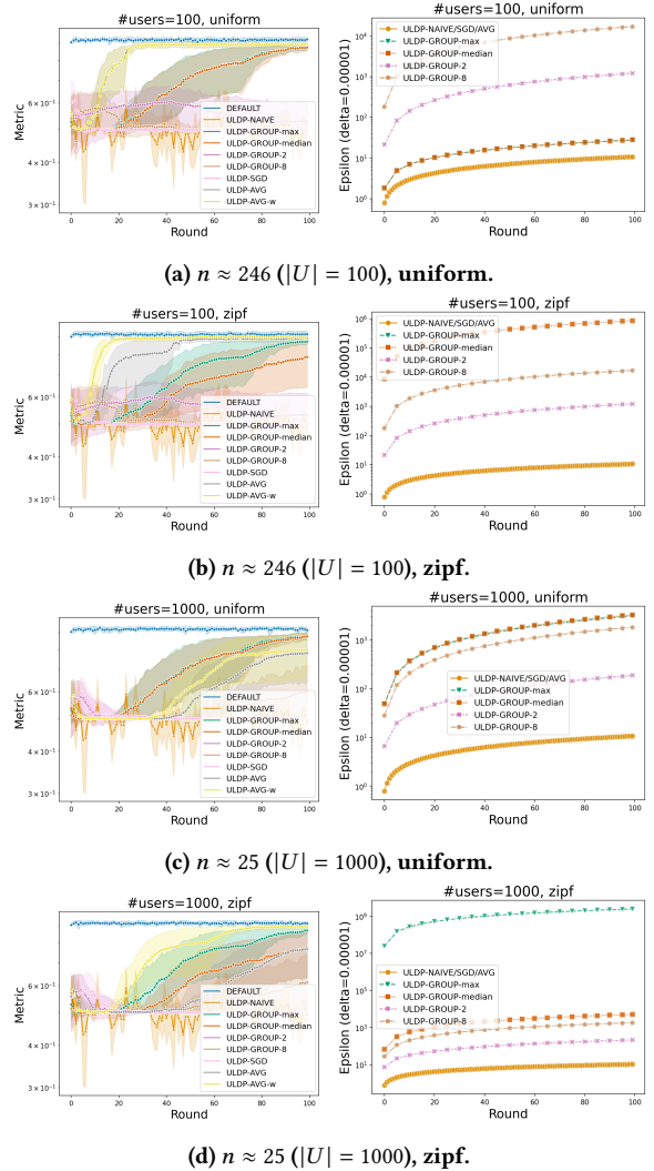
Figure 4: Privacy-utility trade-offs on Credicard dataset: Test Accuracy (Left), Privacy (Right).
