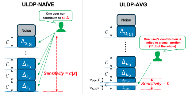
Figure 3: An intuitive illustration of the difference between ULDP-NAIVE and ULDP-AVG. In ULDP-NAIVE, every user can contribute to whole model deltas. In ULDP-AVG, one user's contribution is limited to a small portion, i.e., 1/|U| of the whole model delta, which reduces user-level sensitivity.
