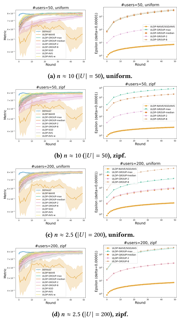
Figure 6: HeartDisease.
