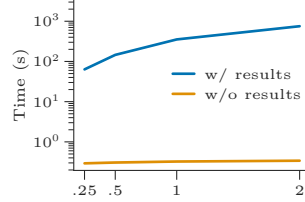
Figure 12: Runtime on GitTables across scaling factors.
