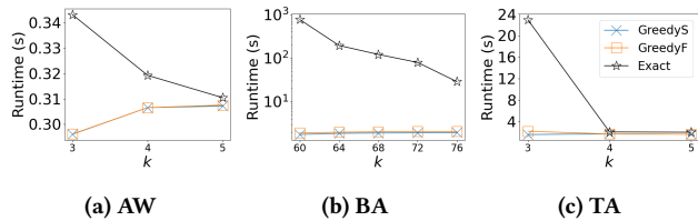
Figure 7: Performance Compared to Exact Solutions
