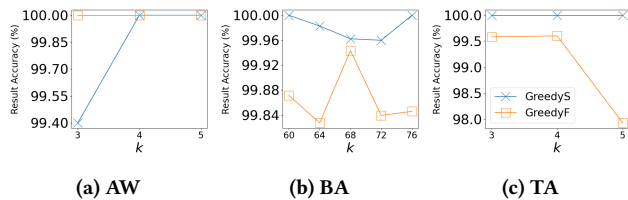
Figure 8: Effectiveness Compared to Exact Solutions
