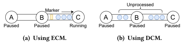
Figure 4: Using ECM, workers A and B have paused when worker C is still waiting for the marker. Using DCM, all workers have paused, leaving in-flight data unprocessed.
