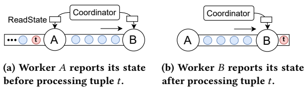
Figure 5: Inconsistent state between workers A and B.
