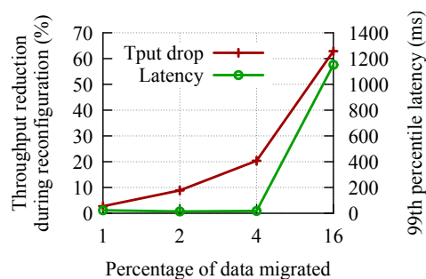
Figure 9: Effect of migrating fractions of the YCSB database.
