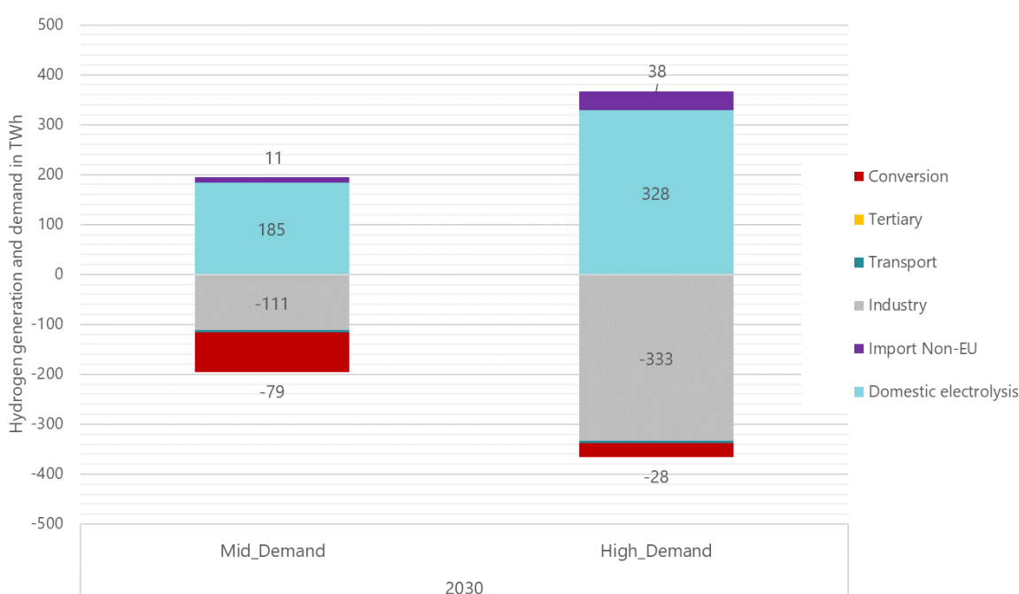
Figure 3.2: European hydrogen balance for 2030.
