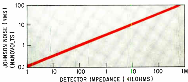
Noise threshold. Typical value of Johnson noise is plotted for a given detector as a function of detector impedance. The choice of operating frequency is arbitrary, as long as the system has a 1-hertz bandwidth.
