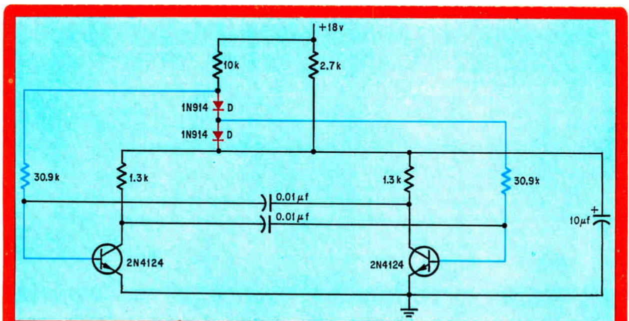
Straight and narrow. Those changes in transistor characteristics that cause the multivibrator frequency circuit to shift are nullified by diodes D_1 and D_2 . The changes in the forward drops of the diodes are nearly the changes in the base-emitter and collector-emitter voltages in the transistors.
