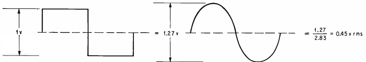
Waveform comparison. Fundamental sine-wave component of a square wave is larger than the square wave.
