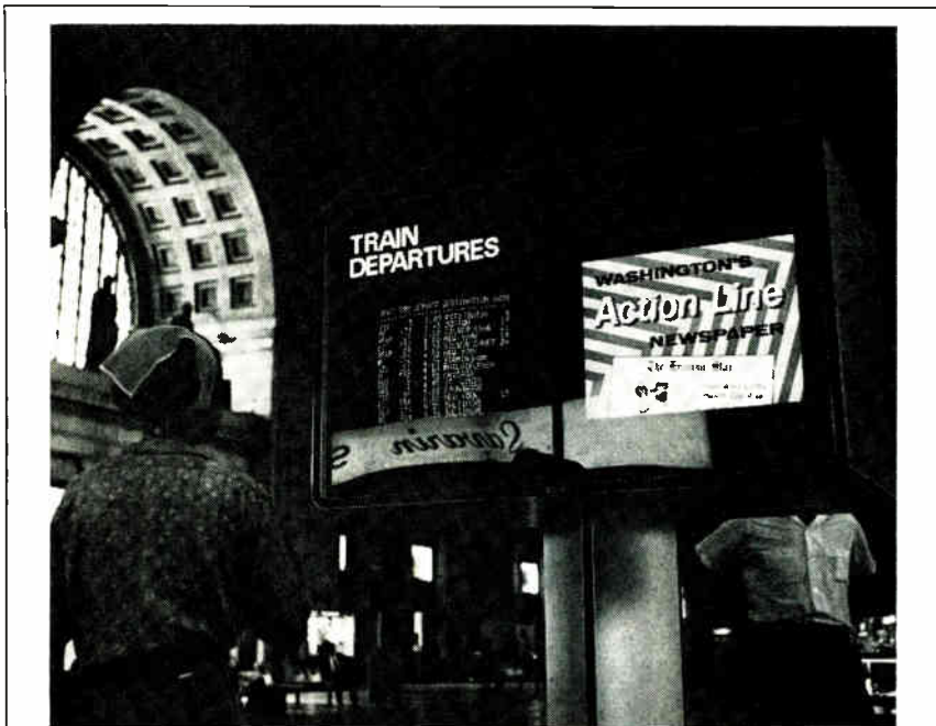
On display. The A.B. Dick Co. has long been known for its duplicating and copying machines. But now, as a result of spin-off from its electrostatic high-speed label-printing equipment, the firm has entered the electronic data-display field with this unit, the Videograph Series 900. It can present up to 512 characters in 16 rows directly from a keyboard or a computer. This installation is at Penn Central Station in Washington.
